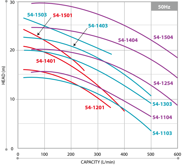
MXM54 Performance curves
